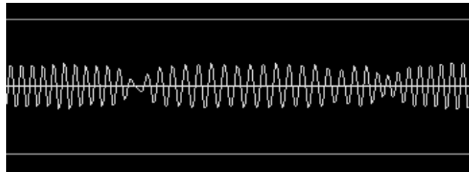
Figure 37.2 AFSK signal
