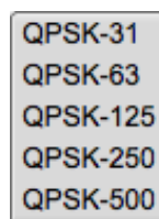
Figure 59.17 QPSK
