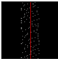
Figure 25.3 DominoEX Mistuned
