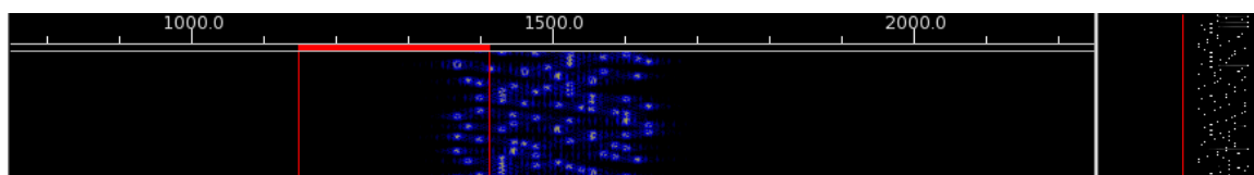
Figure 25.4 DominoEX Mistuned
